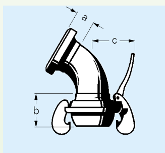
Genuine BAUER HK Bend 60° S12
