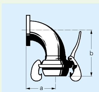
Genuine BAUER HK Flanged Bend 90° with ball S19
