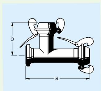
Genuine BAUER HK Tee S21
